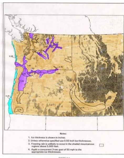
Figure 3-7. 50-Year Recurrence Interval Uniform Ice Thicknesses – Pacific Northwest and Lake Superior (ASCE-7-02 2003a)
